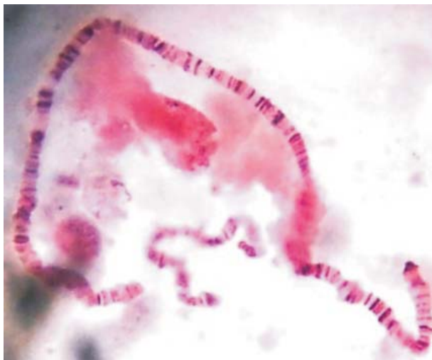
Fig. 5. Chromosome 3 (2L)
